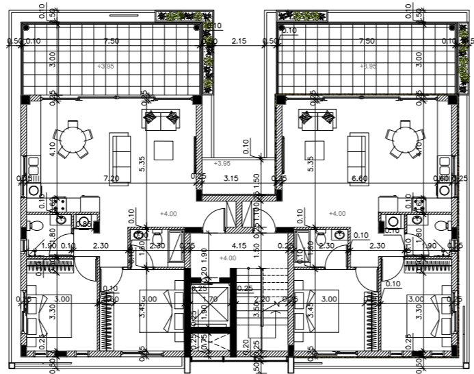
1ST FLOOR
